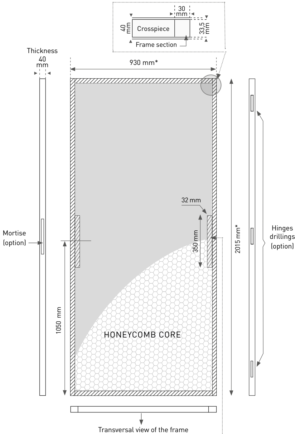
Dimensions board - mm
